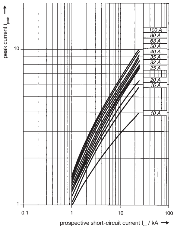
S 700 characteristic K let-through peak current ( I_{peak} )
