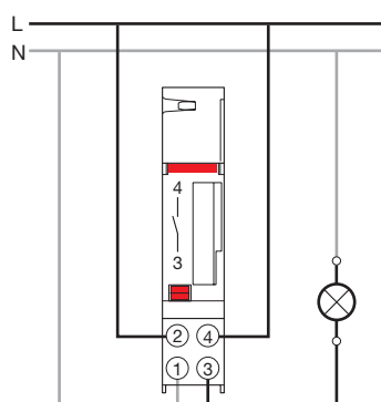
Connection scheme AT1, AT1-R
