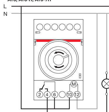
AT3, AT3-R, AT3-7R
