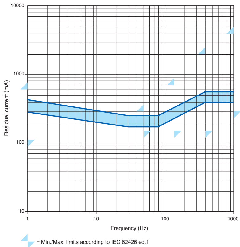
DDA 200 B S type, 300 mA
