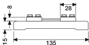
SNT30 ÷ 200 A/60 mV
