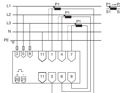
- Indirect connection (through C.T.)
