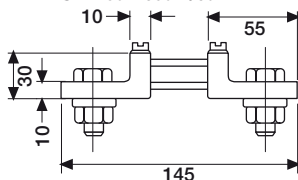
SNT400 ÷ 700 A/60 mV
